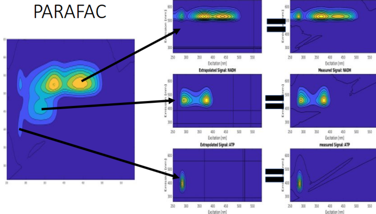
Fig.2: Application of PARAFAC to decompose a mixture ATP, NADH and FAD into the EEMs of its single constituents.
